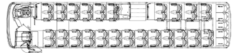
TC12 - Centre door with toilet (51+1+1)
