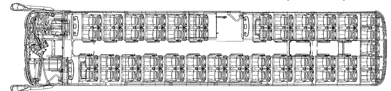
GT12 - Centre door with toilet (53+1+1)
